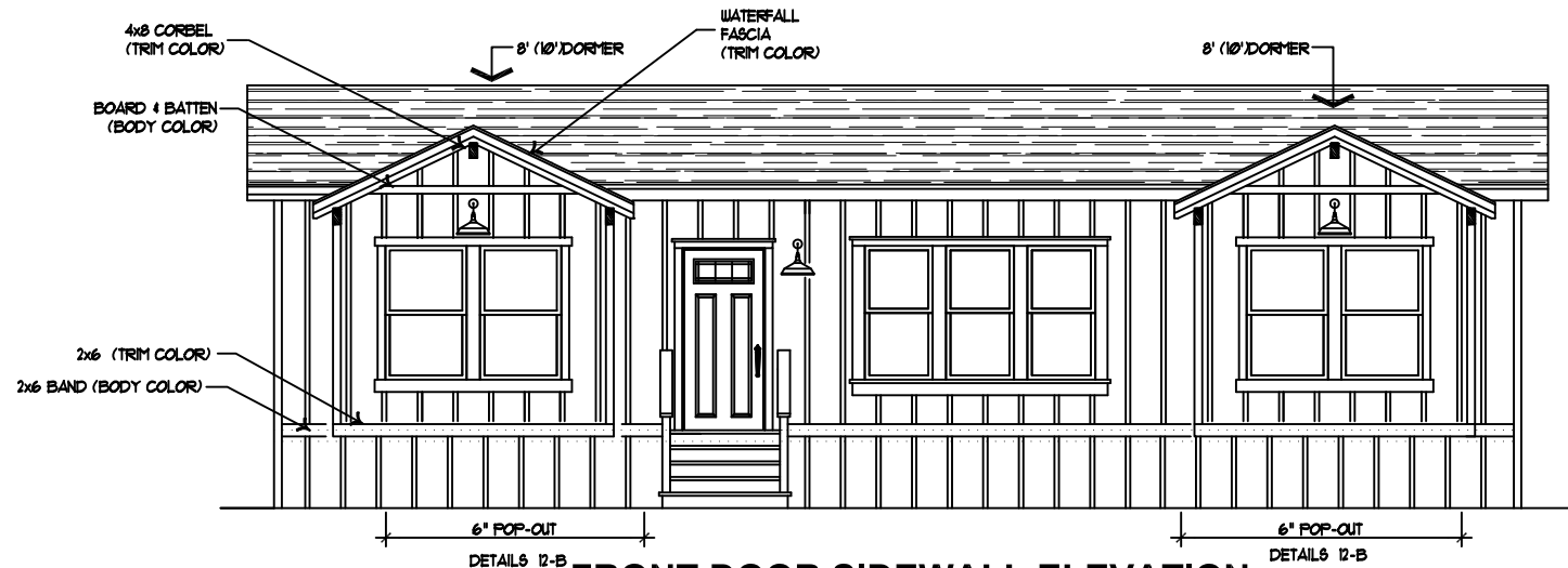
FRONT DOOR SIDEWALL ELEVATION
