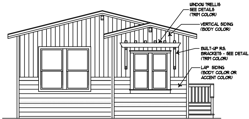
FRONT ENDWALL ELEVATION
