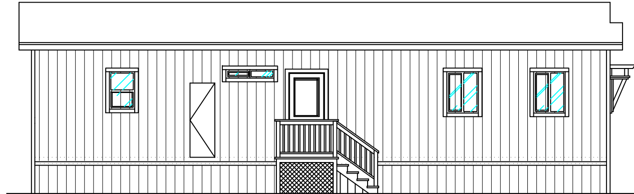
SIDEWALL ELEVATION - RIGHT
