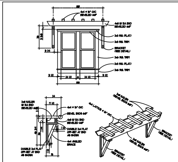
TRELLIS DETAILS
