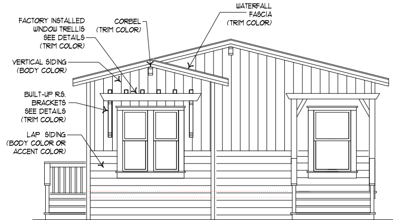
ENDWALL ELEVATION - FRONT (ALT. ENTRY)
