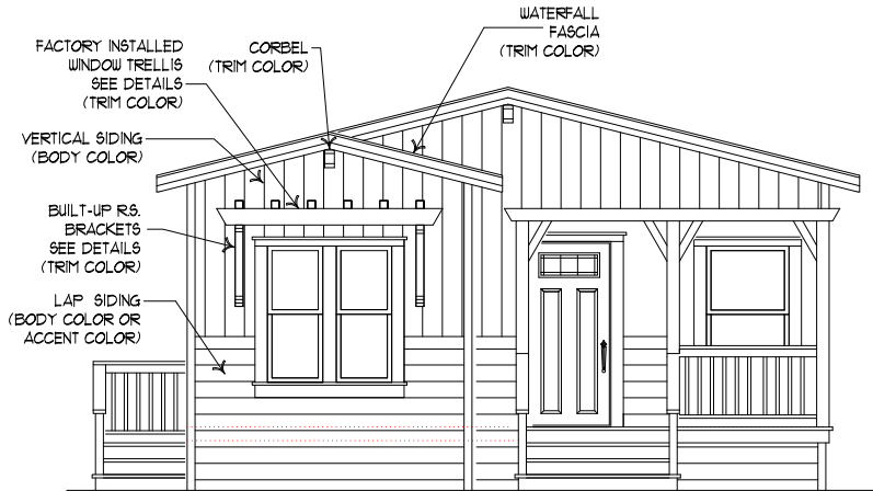
ENDWALL ELEVATION - FRONT (STD)
