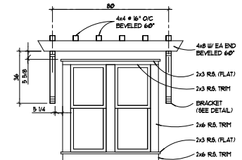
CORONADO TRELLIS WINDOW TRIM DETAIL
