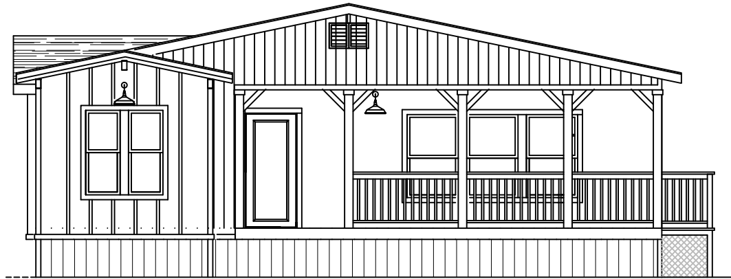
STANDARD FRONT ENDWALL ELEVATION (FOR CLARITY OF ELEVATION, SIDING NOT SHOWN IN PORCH AREA)
